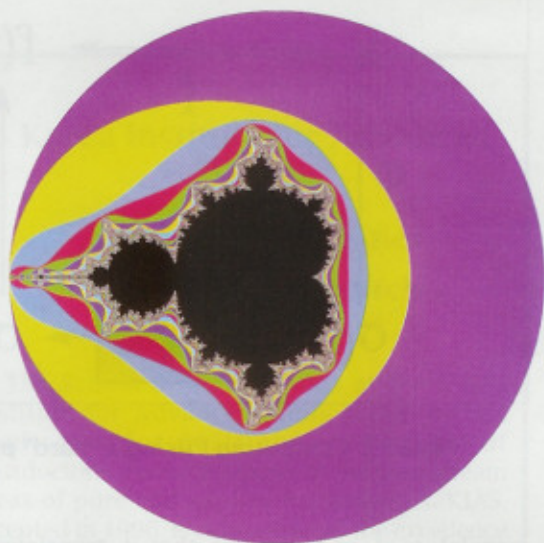
Figure 4. The naïve algorithm for computing M , and some of its outputs.
