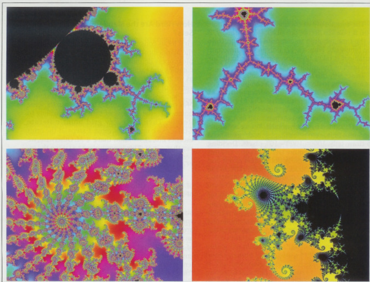
Figure 3. A variety of different images arising in zoom-ins of the Mandelbrot set (in black).
