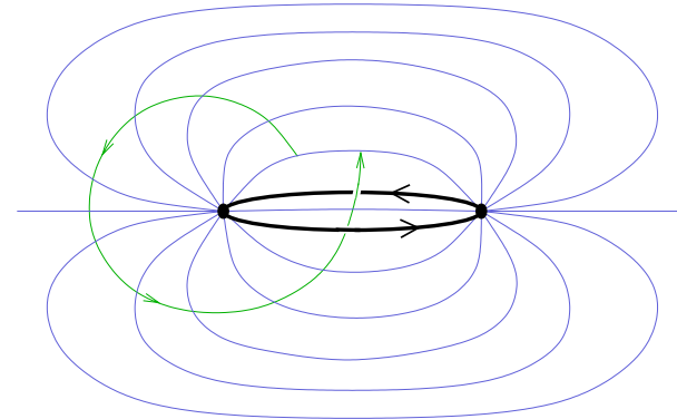
FIGURE 1. An open book decomposition of the tight 3-sphere with one binding orbit and disk-like pages, which are transverse to the Reeb vector field.
