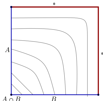
FIGURE 38. Reinterpreting maps I^2 \rightarrow X that satisfy the conditions of (70.1) as paths in the path space P(A, B) from A \cap B to the base point.
