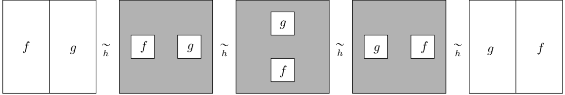
FIGURE 29. The homotopy in the proof of Proposition 54.3.
