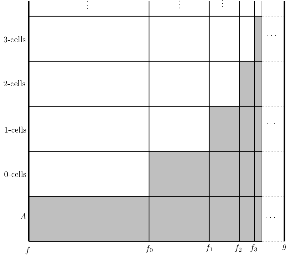
FIGURE 35. A schematic representation of the sequence of maps f_0, f_1, f_2, \dots from X to Y and the homotopy H : X \times I \rightarrow Y constructed in the proof of Lemma 67.12, with the vertical axis representing X (partitioned into A and the unions of cells of various dimensions outside of A ) and the horizontal axis representing the unit interval I . The homotopy is constructed to be independent of the parameter in I on the shaded regions.
