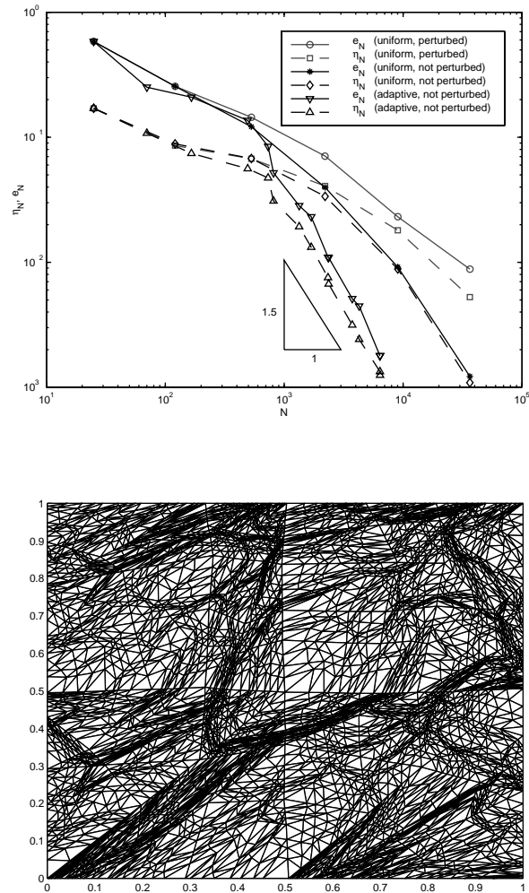
FIGURE 4. Error and error estimator on perturbed meshes for uniform h -refinement and fixed polynomial degree p = 3 in Example 5.2 compared to uniform and h -adaptive mesh-refinement without perturbation (top). Perturbed mesh with 4225 nodes (bottom).
