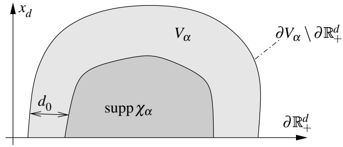
Figure 2.1: The function \chi_\alpha with distance d_0 from the boundary.
