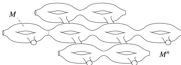
Figure 0.7: A periodic cell M and an approximating submanifold M^n of M^{\text{per}} with n = 8 elements.
