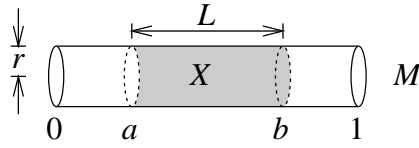
Figure 7.1: The period cell M of the cylinder M^{\text{per}} = \mathbb{R} \times \mathbb{S}^1 .
