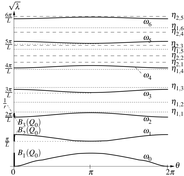
Figure 7.2: The square root of the eigenvalues of the limit operator Q_0^\theta in Case A, B (thick line) and E (dotted and dashed line) plotted for L = 0.5 and r = 1/13 . Here, at least m = 2 gaps occur.
