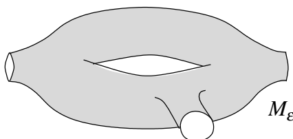
Figure 8.1: A period cell M_\varepsilon with smooth boundary \partial M_\varepsilon . The corresponding periodic manifold M_\varepsilon^{\text{per}} is periodic with respect to a group with r = 2 generators.
