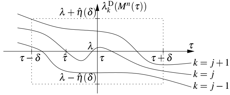
Figure 8.4: The number of eigenvalue branches \lambda_k^{\text{D}}(M^n(\cdot)) crossing the \lambda -level in [\tau - \delta, \tau + \delta] can be estimated by the number of eigenvalue branches in the interval [\lambda - \hat{\eta}(\delta), \lambda + \hat{\eta}(\delta)] at the fixed parameter \tau .
