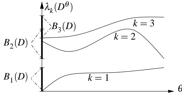
Figure 3.3: Band structure of the spectrum of a \Gamma -periodic operator D . Here, the second and third band overlap.
