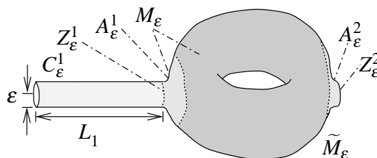
Figure 5.1: Here, the period cell \tilde{M}_\varepsilon is obtained from glueing the cylinder C_\varepsilon^1 of length L_1 > 0 and radius \varepsilon > 0 to the period cell M_\varepsilon constructed in Figure 4.2.
