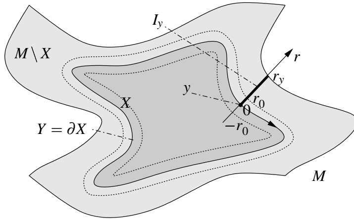
Figure 6.1: Normal coordinates (r, y) parametrising a neighbourhood of Y = \partial X and M \setminus X .
