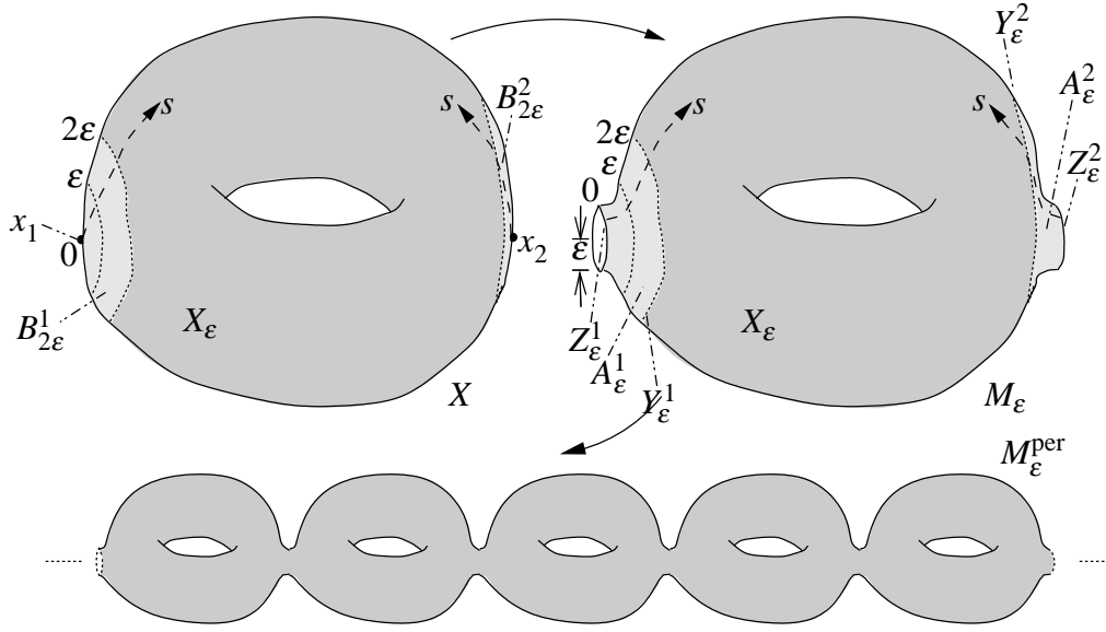
Figure 4.2: Construction of the periodic manifold M_\varepsilon^{\text{per}} . We start with the compact manifold X , modify X in a neighbourhood of x_1, \dots, x_{2r} . Here, the period cell M_\varepsilon has only r = 1 pairs of cylindrical ends. Finally we glue the periodic manifold M_\varepsilon^{\text{per}} from copies of the period cell.
