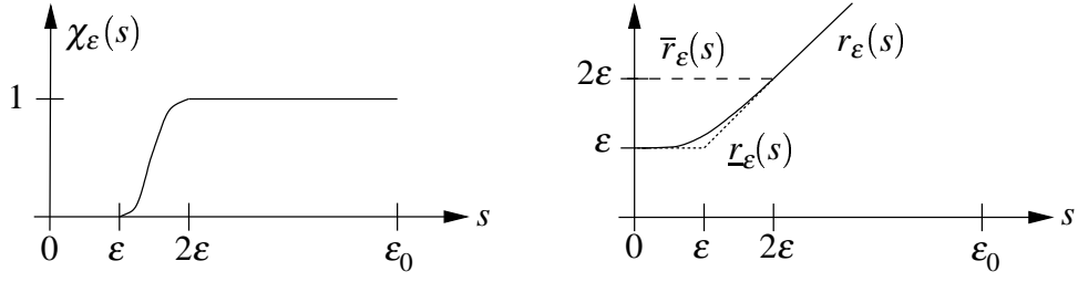
Figure 4.1: Graphs of the cut-off function \chi_\varepsilon and of the radii functions \underline{r}_\varepsilon, r_\varepsilon, \bar{r}_\varepsilon .
