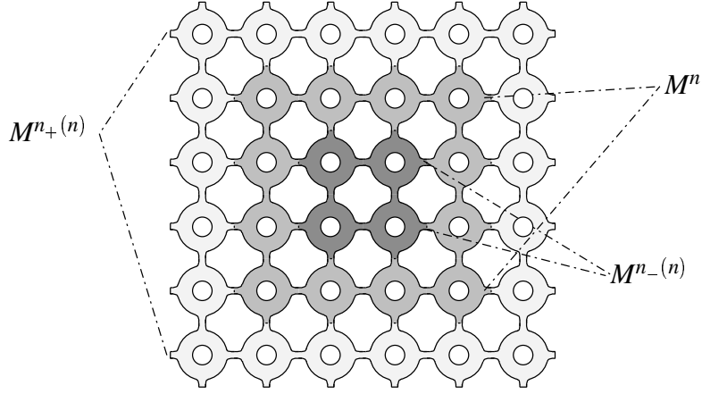
Figure 8.3: Definition of the integers n_+(n) and n_-(n) .
