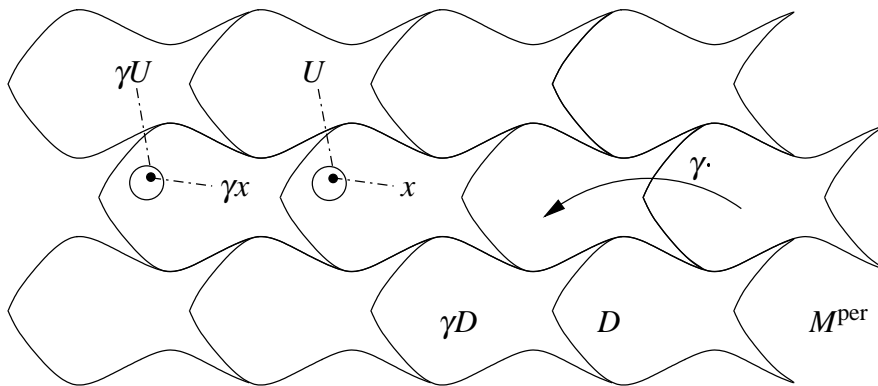
Figure 3.1: The group \Gamma = \mathbb{Z}^2 acting properly discontinuously on M^{\text{per}} . An element \gamma \in \Gamma translates the fundamental domain D to the disjoint copy \gamma D . We call the closure M = \overline{D} a period cell .
