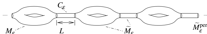
Figure 0.3: A periodic manifold with long thin cylinders obtained by taking M_\varepsilon and C_\varepsilon as new period cell \tilde{M}_\varepsilon .
