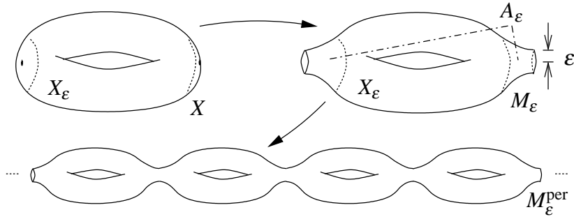
Figure 0.1: Construction of a periodic manifold in Case A.
