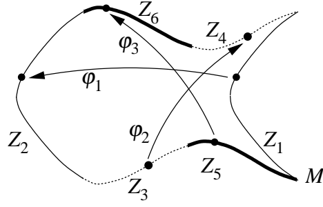
Figure 3.2: A period cell with the isometries \varphi_i identifying elements on the boundary.
