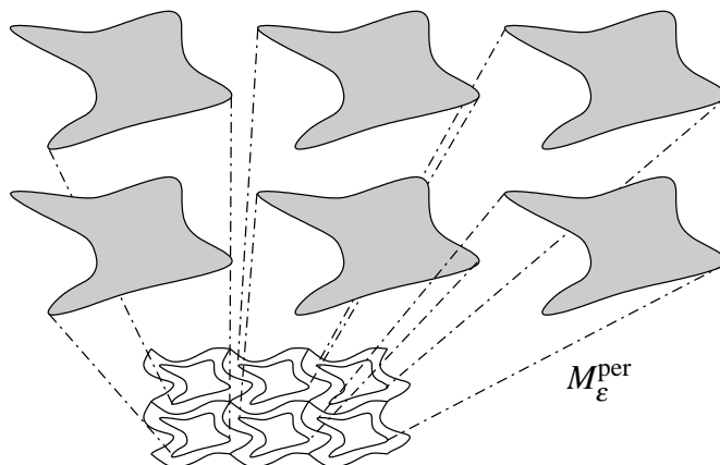
Figure 0.5: An, alas imperfect, attempt to picture the conformally perturbed manifold M_\varepsilon^{\text{per}} obtained by scaling the manifold M^{\text{per}} of Figure 0.4 outside the grey area X^{\text{per}} .
