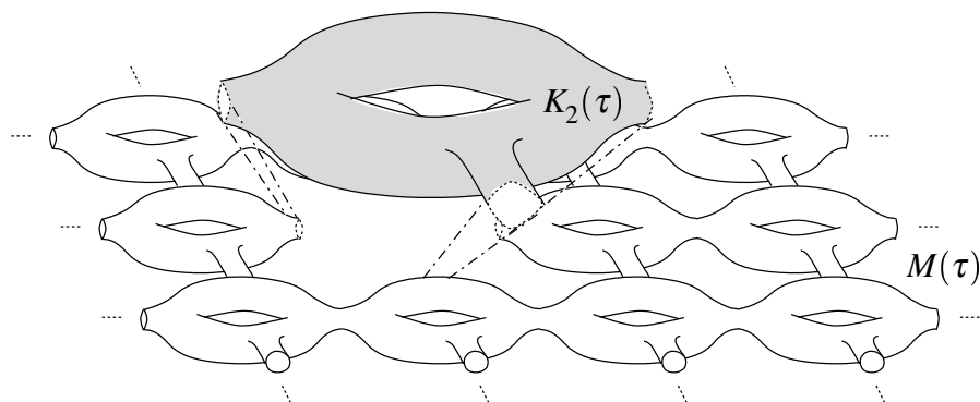
Figure 0.6: The perturbed manifold M(\tau) . Again, this picture is only an attempt since one cannot draw correctly the conformally perturbed area K_1(\tau) \setminus K_2(\tau) where the conformal factor \rho(\tau) is a non-constant function.
