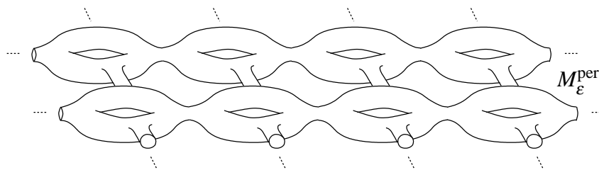
Figure 0.2: A manifold periodic with respect to a group generated by two elements (like \mathbb{Z}^2 or \mathbb{Z} \times \mathbb{Z}_p ).
