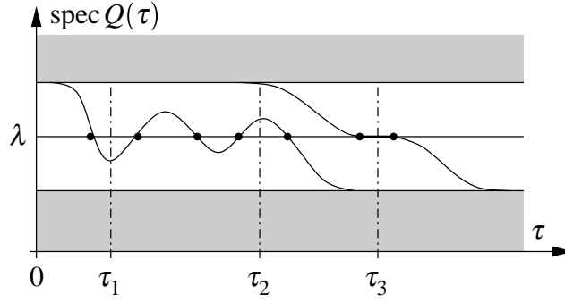
Figure 8.5: Two Eigenvalue branches in a gap of the operator Q(0) . Here, the eigenvalue counting function of (Q(\tau))_\tau satisfies \mathcal{N}_{\tau_1}(Q(\cdot), \lambda) = 1 , \mathcal{N}_{\tau_2}(Q(\cdot), \lambda) = 4 and \mathcal{N}_{\tau_3}(Q(\cdot), \lambda) = \infty . Note that the eigenvalue counting function does not count eigenvalue branches but the number of intersection points of the branches with the level \lambda .
