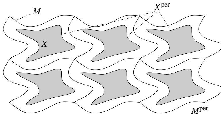
Figure 0.4: In Case B the \mathbb{Z}^2 -periodic manifold M^{\text{per}} is given. We choose a period cell M such that the periodic subset X^{\text{per}} does not intersect the boundary of M . We further suppose that normal coordinates with respect to \partial X are defined on \overline{M \setminus X} .
