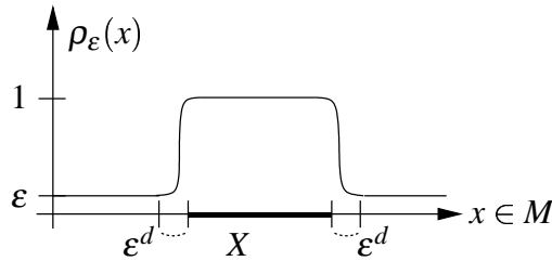
Figure 6.2: The conformal factor \rho_\varepsilon leaving X undeformed.
